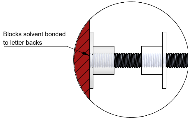
DETAIL DW II SCALE 1:1
