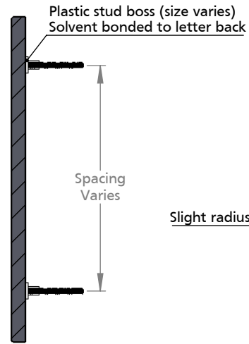
SECTION VIEW A-A II SCALE 1:5
