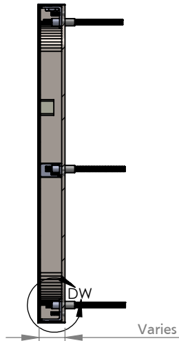
SECTION A-A II SCALE 1:5
